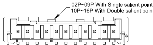
10P-16P SCALE 1:0.8
