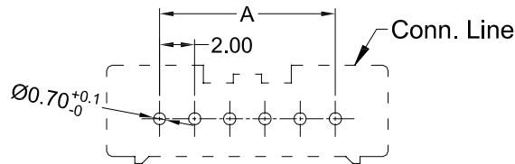
Recommended P.C.B Layout General Tolerance±0.05
