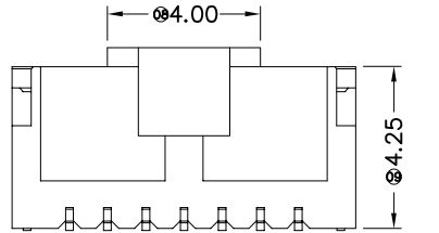
02P~09P Without Gate Location groove
