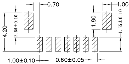
Recommad PCB Layout
