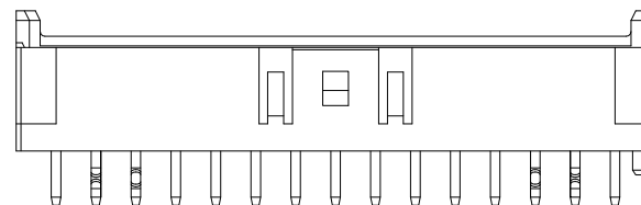
15Pin
