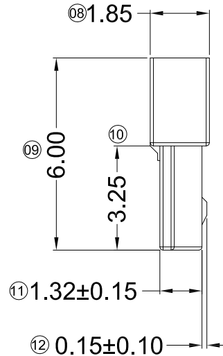
4P~30P Double Salient Scale 1:5
